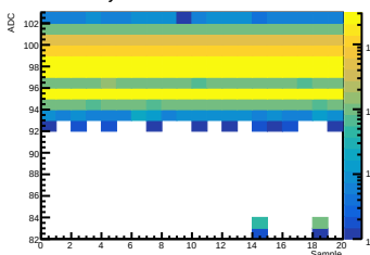
Crystal 12 SiPM 05 Waveform
