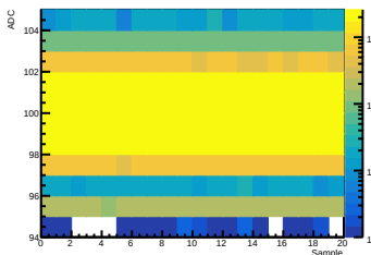
Crystal 12 SiPM 01 Waveform
