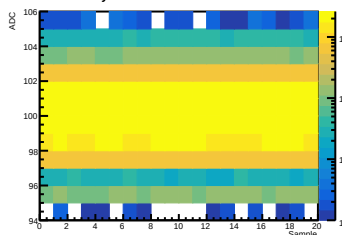
Crystal 12 SiPM 07 Waveform
