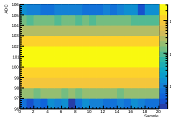
Crystal 12 SiPM 03 Waveform
