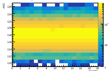
Crystal 12 SiPM 12 Waveform
