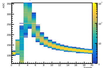
Crystal 12 SiPM 12 Waveform
