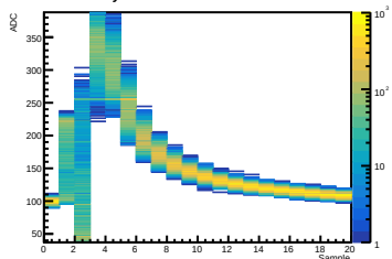
Crystal 12 SiPM 08 Waveform
