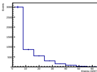
Crystal 12 SIPM 05 Energy
