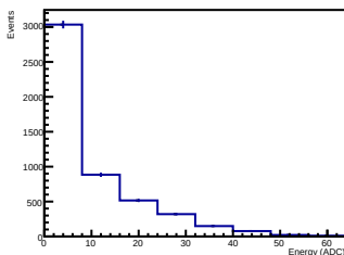
Crystal 12 SIPM 09 Energy
