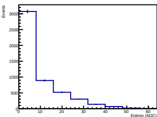
Crystal 12 SIPM 04 Energy
