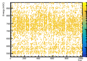
Central Crystal SIPM 5: Energy vs ToA
