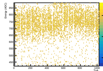
Central Crystal SIPM 11: Energy vs ToA
