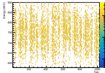
Central Crystal SIPM 1: Energy vs ToA
