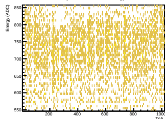
Central Crystal SIPM 12: Energy vs ToA
