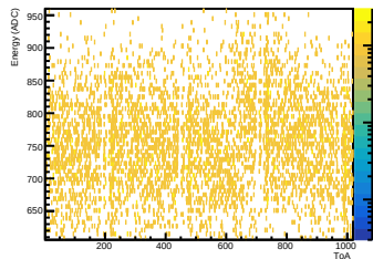
Central Crystal SIPM 2: Energy vs ToA
