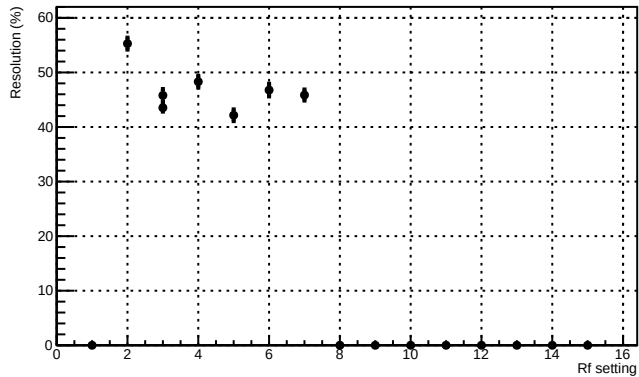
Central resolution vs Rf (V=0.000, CC=12)
