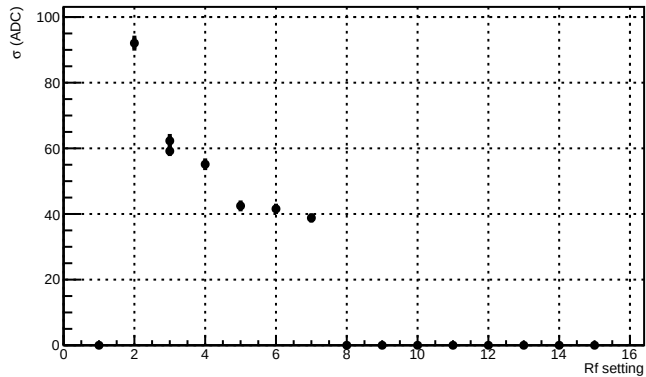
Central \sigma vs CC (V=0.000, Rf=3)
