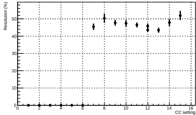
Central resolution vs CC (V=0.000, Rf=3)
