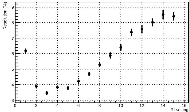
Central resolution vs Rf (V=1.260, CC=12)
