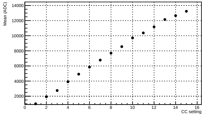
Central mean vs CC (V=1.260, Rf=3)
