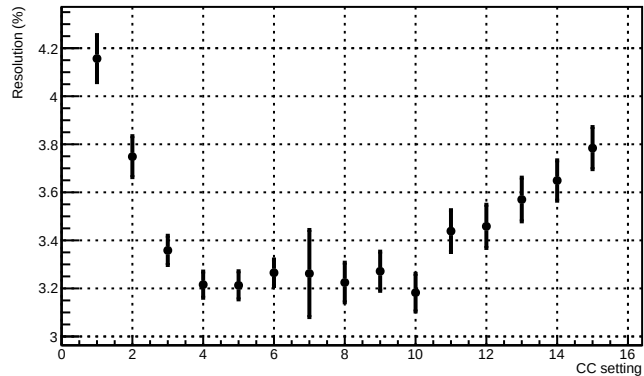
Central resolution vs CC (V=1.260, Rf=3)
