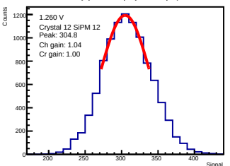
ADC-only | 1.260 V | crystal 12 | sipm 12
