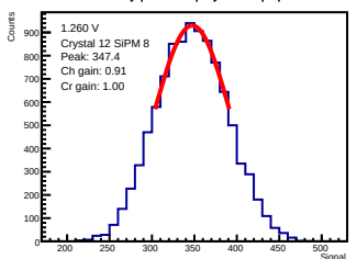
ADC-only | 1.260 V | crystal 12 | sipm 8
