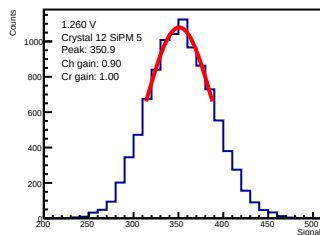
ADC-only | 1.260 V | crystal 12 | sipm 5
