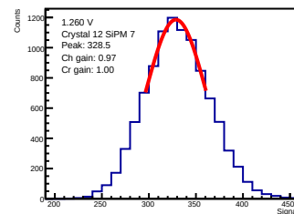
ADC-only | 1.260 V | crystal 12 | sipm 7
