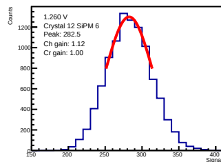
ADC-only | 1.260 V | crystal 12 | sipm 6
