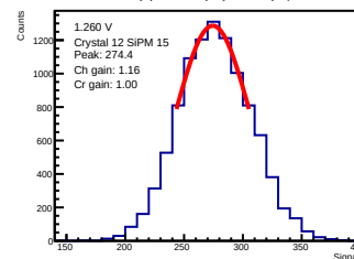
ADC-only | 1.260 V | crystal 12 | sipm 15
