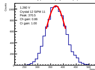
ADC-only | 1.260 V | crystal 12 | sipm 11
