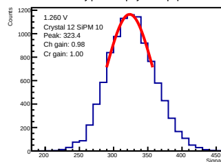
ADC-only | 1.260 V | crystal 12 | sipm 10
