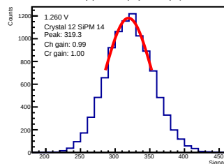
ADC-only | 1.260 V | crystal 12 | sipm 14
