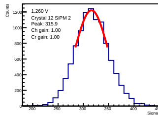
ADC-only | 1.260 V | crystal 12 | sipm 2
