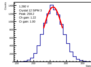
ADC-only | 1.260 V | crystal 12 | sipm 3
