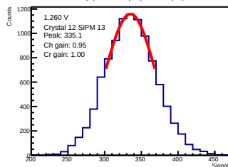
ADC-only | 1.260 V | crystal 12 | sipm 13
