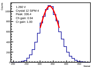
ADC-only | 1.260 V | crystal 12 | sipm 4
