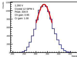
ADC-only | 1.260 V | crystal 12 | sipm 1
