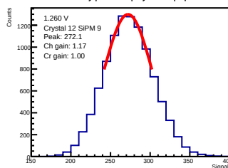
ADC-only | 1.260 V | crystal 12 | sipm 9
