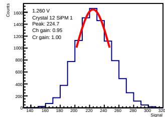
ADC-only | 1.260 V | crystal 12 | sipm 1
