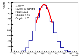
ADC-only | 1.260 V | crystal 12 | sipm 9
