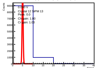
ADC-only | 0.000 V | crystal 12 | sipm 13
