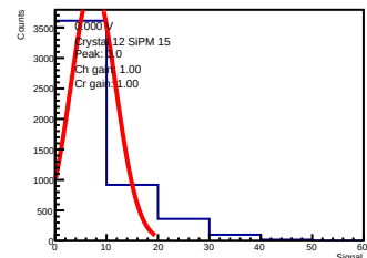
ADC-only | 0.000 V | crystal 12 | sipm 15
