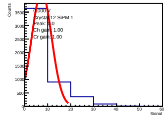
ADC-only | 0.000 V | crystal 12 | sipm 1
