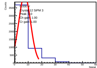
ADC-only | 0.000 V | crystal 12 | sipm 3
