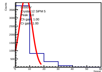
ADC-only | 0.000 V | crystal 12 | sipm 5
