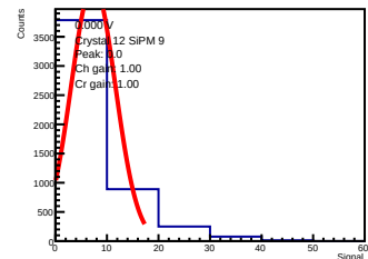
ADC-only | 0.000 V | crystal 12 | sipm 9
