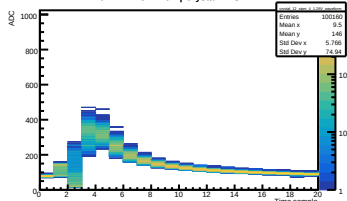
Run 442 Vol 1.26V | Crystal 12 SIPM 4
