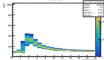
Run 442 Vol 1.26V | Crystal 12 SIPM 7
