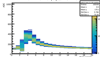
Run 442 Vol 1.26V | Crystal 12 SIPM 13
