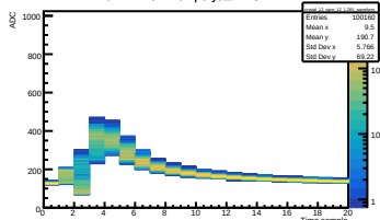
Run 442 Vol 1.26V | Crystal 12 SIPM 12
