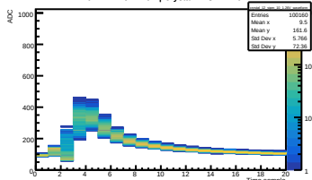
Run 442 Vol 1.26V | Crystal 12 SIPM 10
