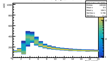
Run 442 Vol 1.26V | Crystal 12 SIPM 5
