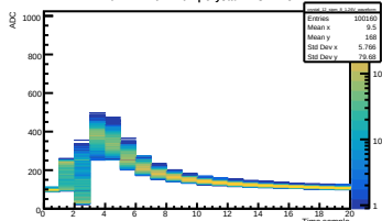
Run 442 Vol 1.26V | Crystal 12 SIPM 8
