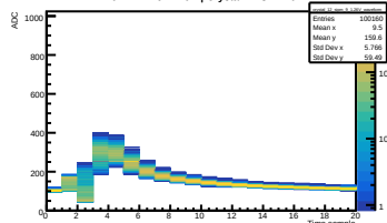
Run 442 Vol 1.26V | Crystal 12 SIPM 9
