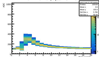
Run 442 Vol 1.26V | Crystal 12 SIPM 15
