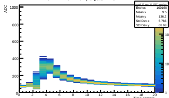
Run 442 Vol 1.26V | Crystal 12 SIPM 14
