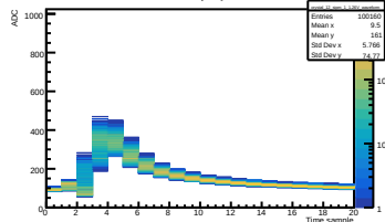
Run 442 Vol 1.26V | Crystal 12 SIPM 1
