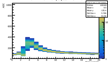
Run 442 Vol 1.26V | Crystal 12 SIPM 6
