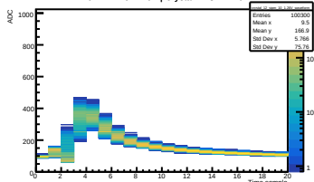
Run 444 Vol 1.26V | Crystal 12 SiPM 10
