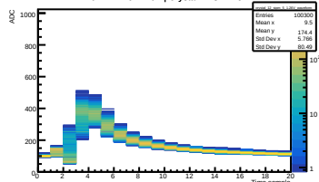
Run 444 Vol 1.26V | Crystal 12 SiPM 5
