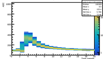
Run 444 Vol 1.26V | Crystal 12 SiPM 2
