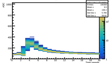
Run 444 Vol 1.26V | Crystal 12 SiPM 3
