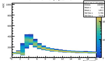
Run 444 Vol 1.26V | Crystal 12 SiPM 14
