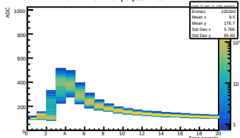
Run 444 Vol 1.26V | Crystal 12 SiPM 11
