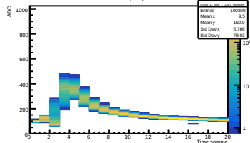
Run 444 Vol 1.26V | Crystal 12 SiPM 1
