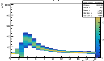
Run 444 Vol 1.26V | Crystal 12 SiPM 4
