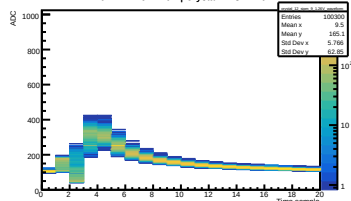
Run 444 Vol 1.26V | Crystal 12 SiPM 9
