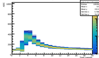
Run 446 Vol 1.26V | Crystal 12 SIPM 2
