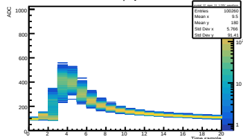
Run 446 Vol 1.26V | Crystal 12 SIPM 11
