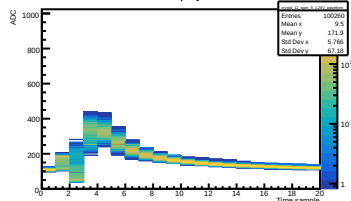
Run 446 Vol 1.26V | Crystal 12 SIPM 9
