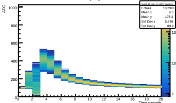
Run 446 Vol 1.26V | Crystal 12 SIPM 8
