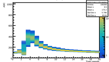
Run 446 Vol 1.26V | Crystal 12 SIPM 1
