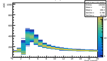
Run 446 Vol 1.26V | Crystal 12 SIPM 5
