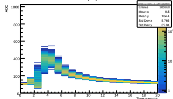
Run 446 Vol 1.26V | Crystal 12 SIPM 13
