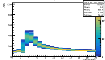
Run 446 Vol 1.26V | Crystal 12 SIPM 7
