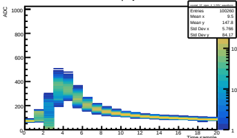
Run 446 Vol 1.26V | Crystal 12 SIPM 4
