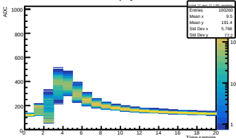
Run 446 Vol 1.26V | Crystal 12 SIPM 12
