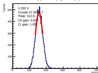
ADC-only | 1.250 V | crystal 12 | sipm 7
