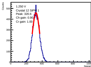
ADC-only | 1.250 V | crystal 12 | sipm 1
