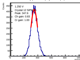
ADC-only | 1.250 V | crystal 12 | sipm 11
