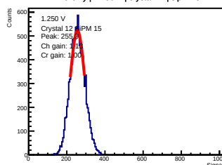
ADC-only | 1.250 V | crystal 12 | sipm 15
