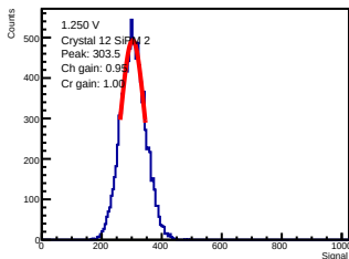
ADC-only | 1.250 V | crystal 12 | sipm 2
