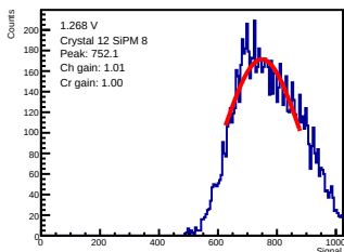
ADC-only | 1.268 V | crystal 12 | sipm 8
