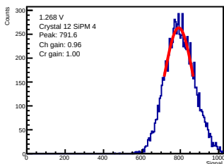
ADC-only | 1.268 V | crystal 12 | sipm 4
