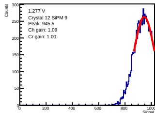
ADC-only | 1.277 V | crystal 12 | sipm 9
