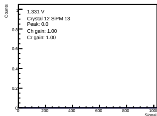
ADC-only | 1.331 V | crystal 12 | sipm 13
