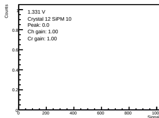
ADC-only | 1.331 V | crystal 12 | sipm 10
