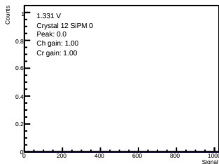
ADC-only | 1.331 V | crystal 12 | sipm 0
