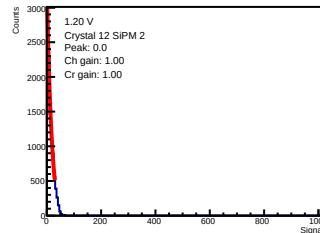
ADC-only | 1.20 V | crystal 12 | sipm 2
