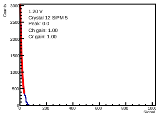
ADC-only | 1.20 V | crystal 12 | sipm 5
