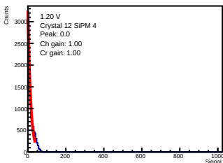
ADC-only | 1.20 V | crystal 12 | sipm 4
