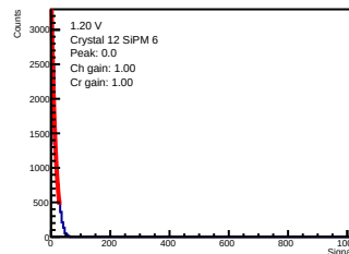
ADC-only | 1.20 V | crystal 12 | sipm 6
