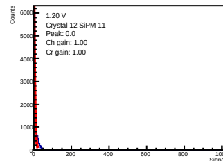
ADC-only | 1.20 V | crystal 12 | sipm 11
