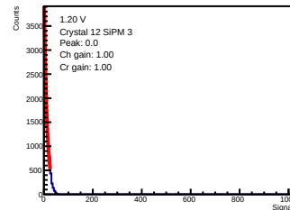
ADC-only | 1.20 V | crystal 12 | sipm 3
