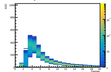
Crystal 12 SiPM 04 Waveform
