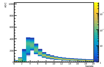
Crystal 12 SiPM 00 Waveform
