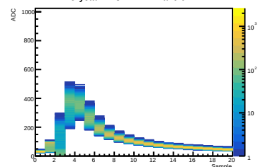
Crystal 12 SiPM 12 Waveform
