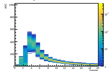
Crystal 12 SiPM 08 Waveform
