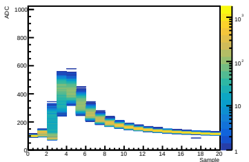
Crystal 12 SiPM 01 Waveform
