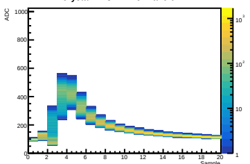
Crystal 12 SiPM 13 Waveform
