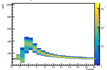
Crystal 12 SiPM 09 Waveform
