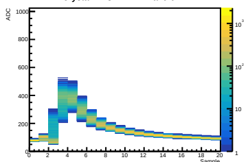
Crystal 12 SiPM 14 Waveform
