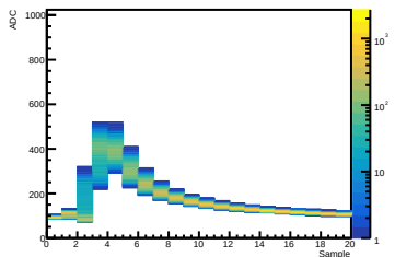
Crystal 12 SiPM 02 Waveform
