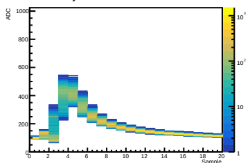
Crystal 12 SiPM 10 Waveform
