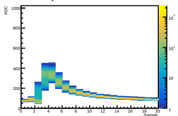
Crystal 12 SiPM 06 Waveform
