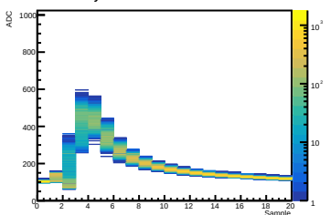
Crystal 12 SiPM 05 Waveform
