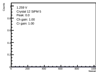
ADC-only | 1.259 V | crystal 12 | sipm 5
