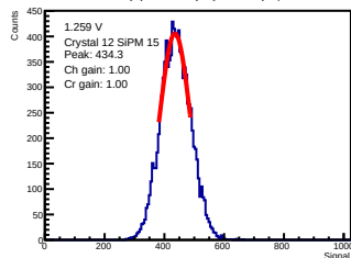
ADC-only | 1.259 V | crystal 12 | sipm 15
