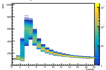
Crystal 12 SiPM 10 Waveform
