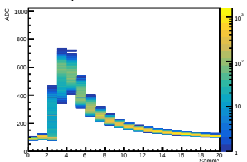
Crystal 12 SiPM 07 Waveform
