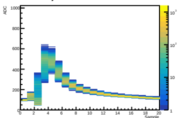
Crystal 12 SiPM 09 Waveform
