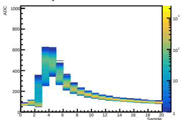
Crystal 12 SiPM 06 Waveform
