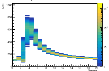
Crystal 12 SiPM 05 Waveform
