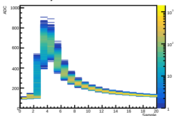
Crystal 12 SiPM 11 Waveform
