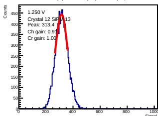
ADC-only | 1.250 V | crystal 12 | sipm 13
