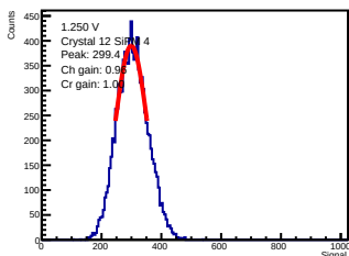
ADC-only | 1.250 V | crystal 12 | sipm 4
