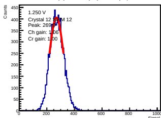
ADC-only | 1.250 V | crystal 12 | sipm 12
