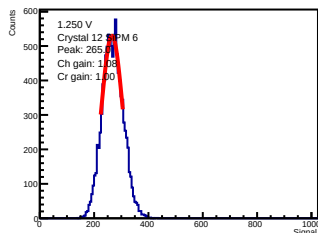
ADC-only | 1.250 V | crystal 12 | sipm 6
