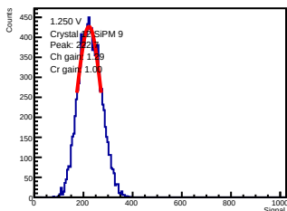
ADC-only | 1.250 V | crystal 12 | sipm 9
