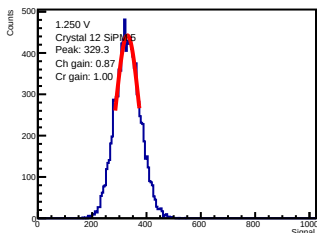
ADC-only | 1.250 V | crystal 12 | sipm 5
