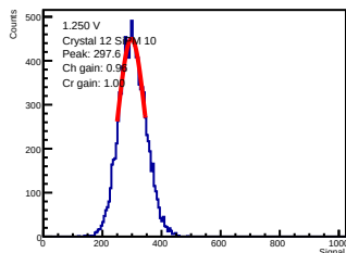
ADC-only | 1.250 V | crystal 12 | sipm 10
