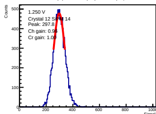
ADC-only | 1.250 V | crystal 12 | sipm 14
