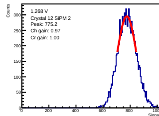
ADC-only | 1.268 V | crystal 12 | sipm 2
