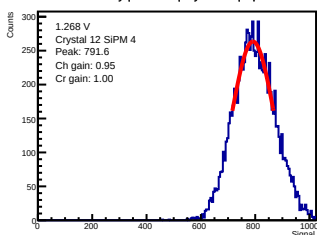
ADC-only | 1.268 V | crystal 12 | sipm 4
