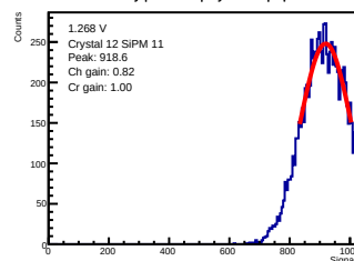
ADC-only | 1.268 V | crystal 12 | sipm 11
