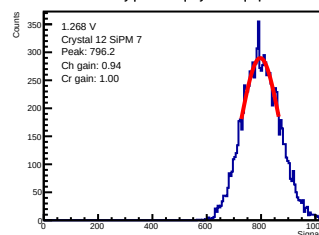
ADC-only | 1.268 V | crystal 12 | sipm 7
