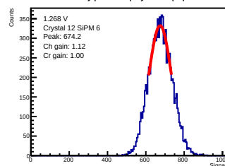
ADC-only | 1.268 V | crystal 12 | sipm 6
