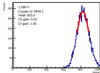
ADC-only | 1.268 V | crystal 12 | sipm 1
