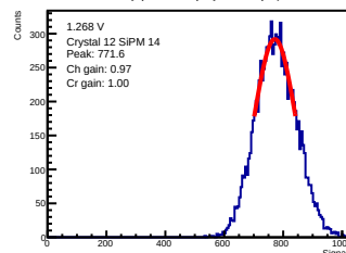
ADC-only | 1.268 V | crystal 12 | sipm 14
