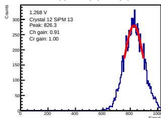
ADC-only | 1.268 V | crystal 12 | sipm 13
