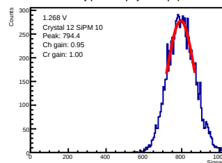
ADC-only | 1.268 V | crystal 12 | sipm 10
