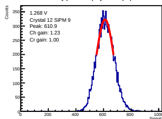
ADC-only | 1.268 V | crystal 12 | sipm 9
