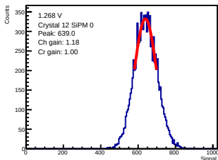
ADC-only | 1.268 V | crystal 12 | sipm 0
