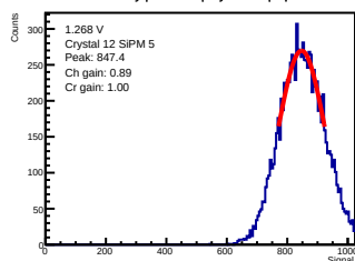
ADC-only | 1.268 V | crystal 12 | sipm 5
