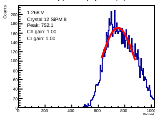
ADC-only | 1.268 V | crystal 12 | sipm 8
