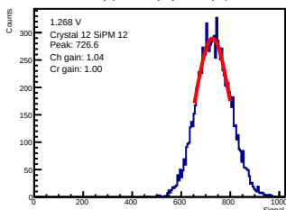
ADC-only | 1.268 V | crystal 12 | sipm 12
