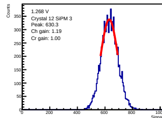
ADC-only | 1.268 V | crystal 12 | sipm 3
