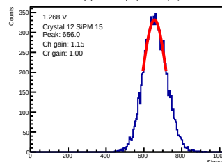
ADC-only | 1.268 V | crystal 12 | sipm 15
