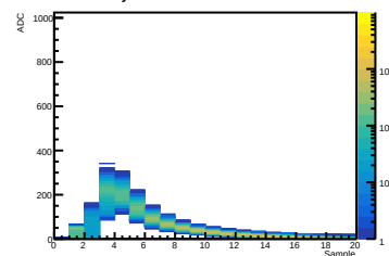
Crystal 12 SiPM 04 Waveform
