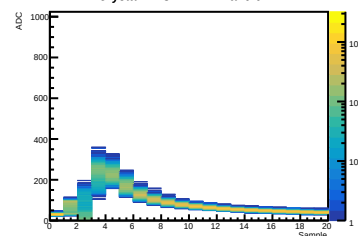
Crystal 12 SiPM 12 Waveform
