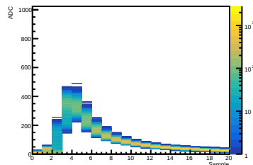
Crystal 12 SiPM 01 Waveform
