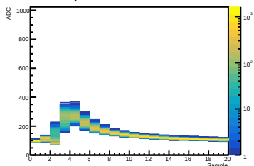
Crystal 12 SiPM 15 Waveform
