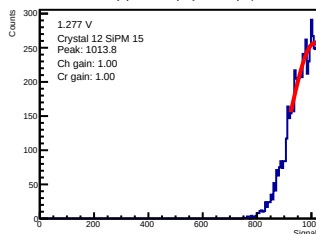
ADC-only | 1.277 V | crystal 12 | sipm 15
