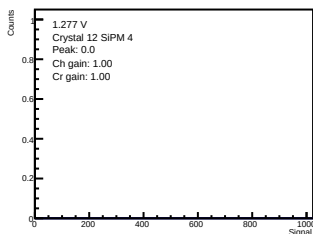
ADC-only | 1.277 V | crystal 12 | sipm 4
