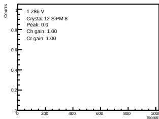
ADC-only | 1.286 V | crystal 12 | sipm 8
