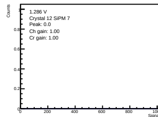
ADC-only | 1.286 V | crystal 12 | sipm 7
