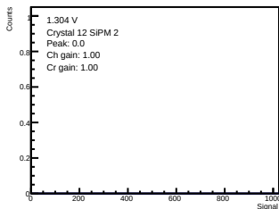
ADC-only | 1.304 V | crystal 12 | sipm 2
