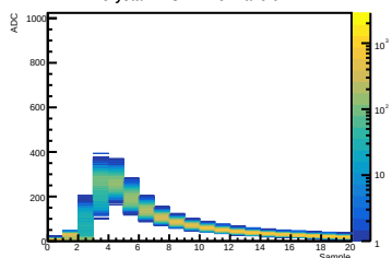
Crystal 12 SiPM 15 Waveform
