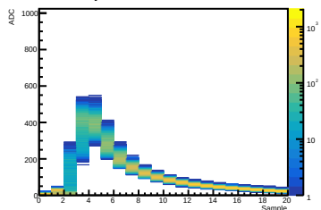
Crystal 12 SiPM 15 Waveform
