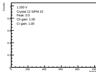
ADC-only | 1.250 V | crystal 12 | sipm 10
