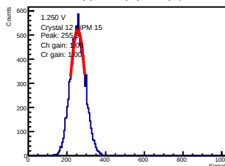
ADC-only | 1.250 V | crystal 12 | sipm 15
