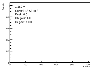
ADC-only | 1.250 V | crystal 12 | sipm 8
