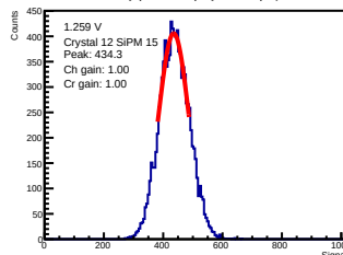
ADC-only | 1.259 V | crystal 12 | sipm 15
