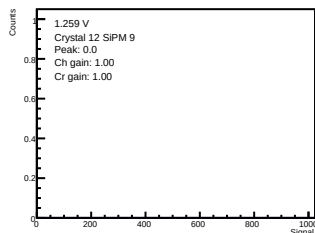
ADC-only | 1.259 V | crystal 12 | sipm 9
