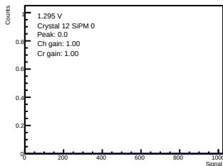
ADC-only | 1.295 V | crystal 12 | sipm 0
