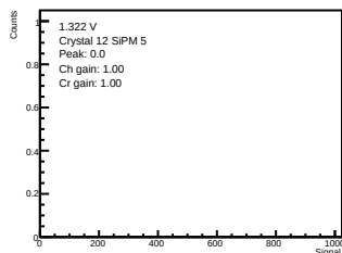
ADC-only | 1.322 V | crystal 12 | sipm 5
