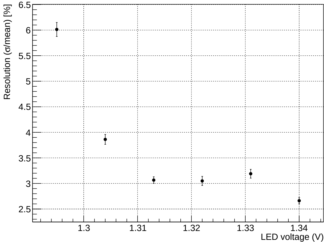
ToT resolution vs LED voltage
