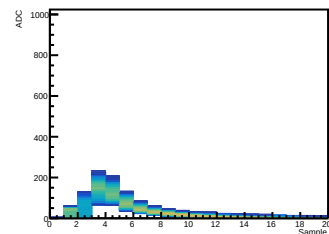
Crystal 12 SiPM 04 Waveform
