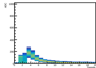
Crystal 12 SiPM 08 Waveform
