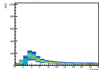
Crystal 12 SiPM 12 Waveform
