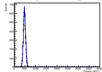
Crystal 12 SiPM 15 Energy
