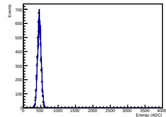
Crystal 12 SiPM 03 Energy
