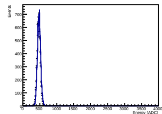
Crystal 12 SiPM 07 Energy
