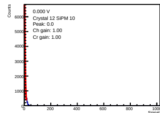
ADC-only | 0.000 V | crystal 12 | sipm 10
