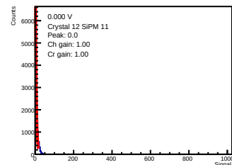
ADC-only | 0.000 V | crystal 12 | sipm 11
