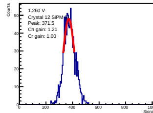
ADC-only | 1.260 V | crystal 12 | sipm 3
