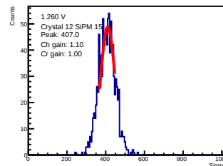
ADC-only | 1.260 V | crystal 12 | sipm 15
