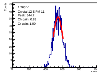
ADC-only | 1.260 V | crystal 12 | sipm 11
