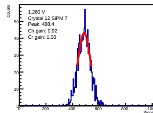
ADC-only | 1.260 V | crystal 12 | sipm 7
