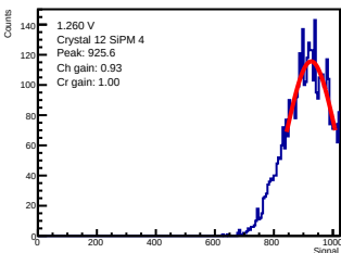
ADC-only | 1.260 V | crystal 12 | sipm 4
