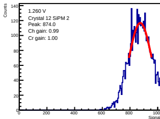
ADC-only | 1.260 V | crystal 12 | sipm 2
