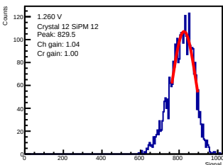
ADC-only | 1.260 V | crystal 12 | sipm 12
