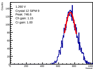
ADC-only | 1.260 V | crystal 12 | sipm 9
