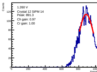
ADC-only | 1.260 V | crystal 12 | sipm 14
