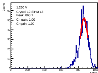
ADC-only | 1.260 V | crystal 12 | sipm 13
