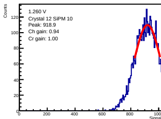
ADC-only | 1.260 V | crystal 12 | sipm 10
