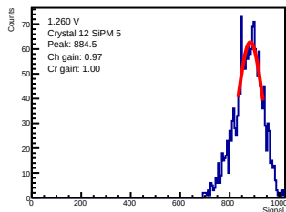
ADC-only | 1.260 V | crystal 12 | sipm 5
