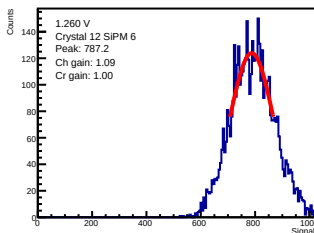
ADC-only | 1.260 V | crystal 12 | sipm 6
