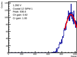
ADC-only | 1.260 V | crystal 12 | sipm 1
