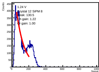
ADC-only | 1.24 V | crystal 12 | sipm 8
