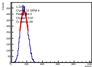
ADC-only | 1.24 V | crystal 12 | sipm 4
