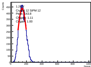
ADC-only | 1.24 V | crystal 12 | sipm 12
