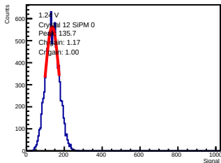
ADC-only | 1.24 V | crystal 12 | sipm 0
