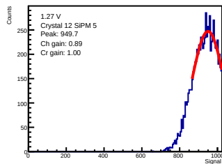
ADC-only | 1.27 V | crystal 12 | sipm 5
