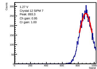
ADC-only | 1.27 V | crystal 12 | sipm 7
