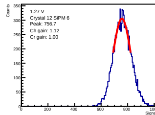
ADC-only | 1.27 V | crystal 12 | sipm 6
