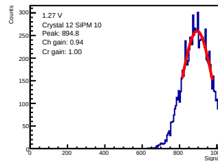
ADC-only | 1.27 V | crystal 12 | sipm 10
