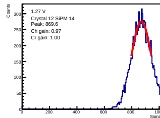
ADC-only | 1.27 V | crystal 12 | sipm 14
