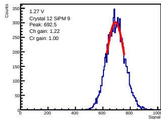
ADC-only | 1.27 V | crystal 12 | sipm 9
