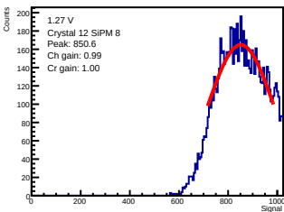
ADC-only | 1.27 V | crystal 12 | sipm 8
