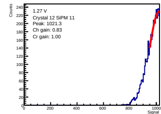
ADC-only | 1.27 V | crystal 12 | sipm 11
