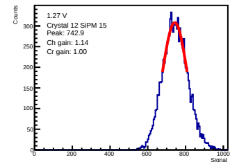
ADC-only | 1.27 V | crystal 12 | sipm 15
