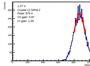
ADC-only | 1.27 V | crystal 12 | sipm 2
