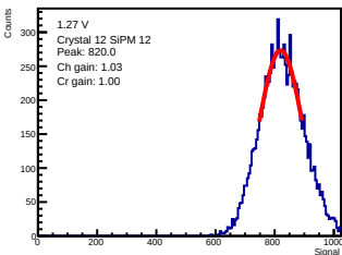
ADC-only | 1.27 V | crystal 12 | sipm 12
