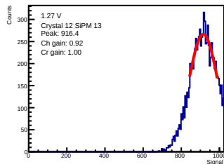
ADC-only | 1.27 V | crystal 12 | sipm 13
