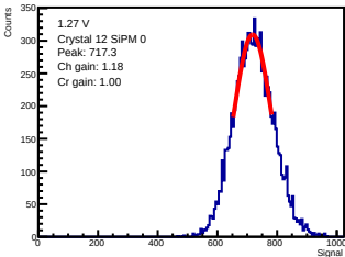
ADC-only | 1.27 V | crystal 12 | sipm 0
