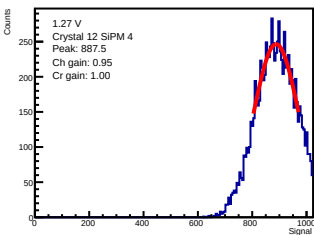
ADC-only | 1.27 V | crystal 12 | sipm 4
