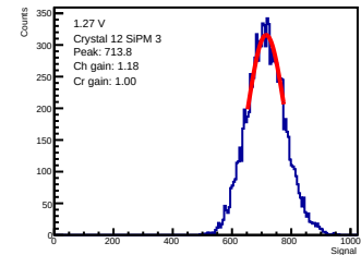
ADC-only | 1.27 V | crystal 12 | sipm 3
