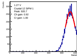
ADC-only | 1.27 V | crystal 12 | sipm 1
