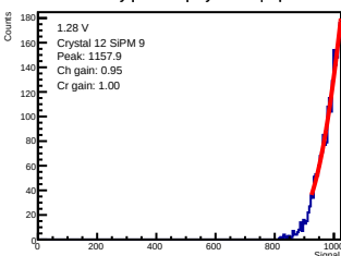
ADC-only | 1.28 V | crystal 12 | sipm 9
