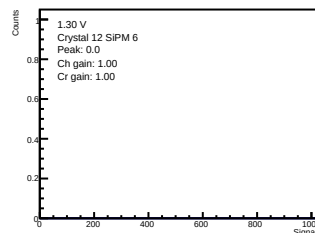
ADC-only | 1.30 V | crystal 12 | sipm 6
