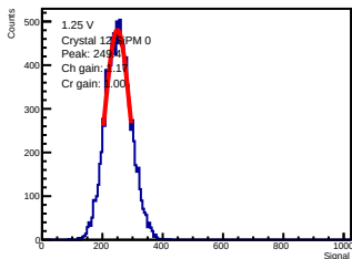
ADC-only | 1.25 V | crystal 12 | sipm 0
