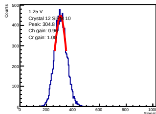
ADC-only | 1.25 V | crystal 12 | sipm 10
