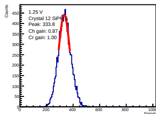
ADC-only | 1.25 V | crystal 12 | sipm 5
