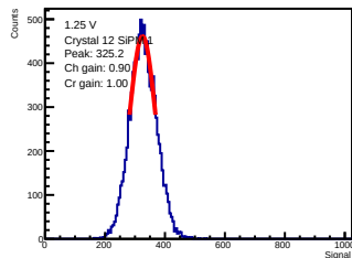
ADC-only | 1.25 V | crystal 12 | sipm 1
