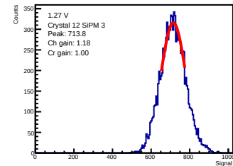
ADC-only | 1.27 V | crystal 12 | sipm 3
