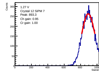
ADC-only | 1.27 V | crystal 12 | sipm 7
