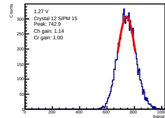
ADC-only | 1.27 V | crystal 12 | sipm 15
