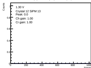
ADC-only | 1.30 V | crystal 12 | sipm 13
